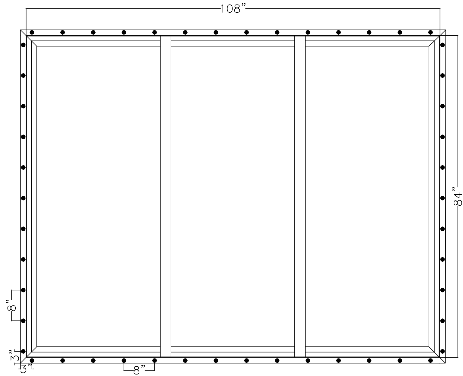
3540 Triple Single Hung WINDOW – FIN INSTALLATION MAXIMUM SIZE 108" X 84" DESIGN PRESSURE +/- 35 PSF
