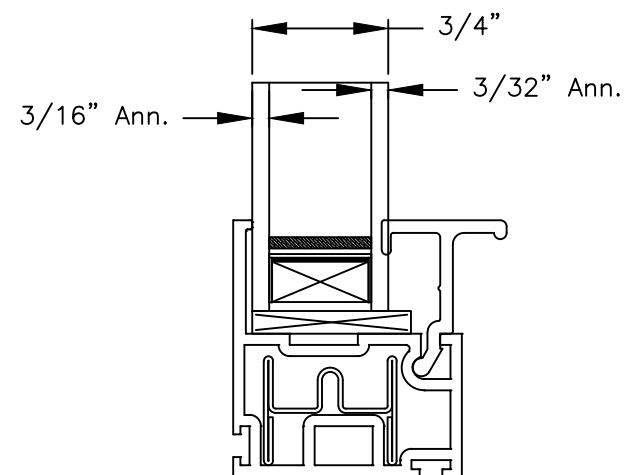
GLAZING DETAIL
